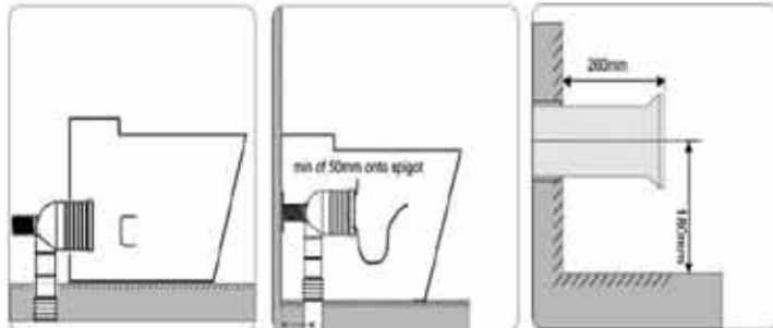
4 Align the pan back to the wall. 5 Connect pan spigot to pan collar. 6 Set up waste pipe and make sure the pipe is parallel to the floor.
