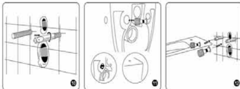
10 Align and push fully assembled toilet back to the wall. 11 Install ceramic cistern. 12 position stop tap then connect rear water inlet valve to stop tap.
