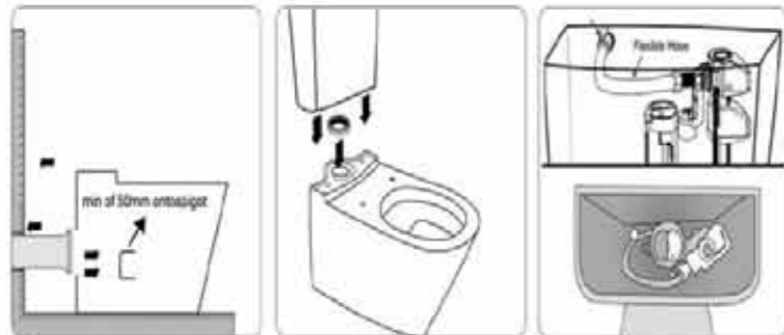
10 Align and push fully assembled toilet back to the wall. 11 Install ceramic cistern. 12 position stop tap then connect rear water inlet valve to stop tap.
