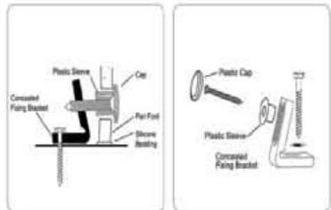
13 Connect the pan with foundation bolt. 14 Fix the pan by screwing the foundation bolt to the floor.
